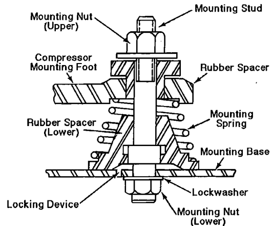
Figure 5. Spring Mount
