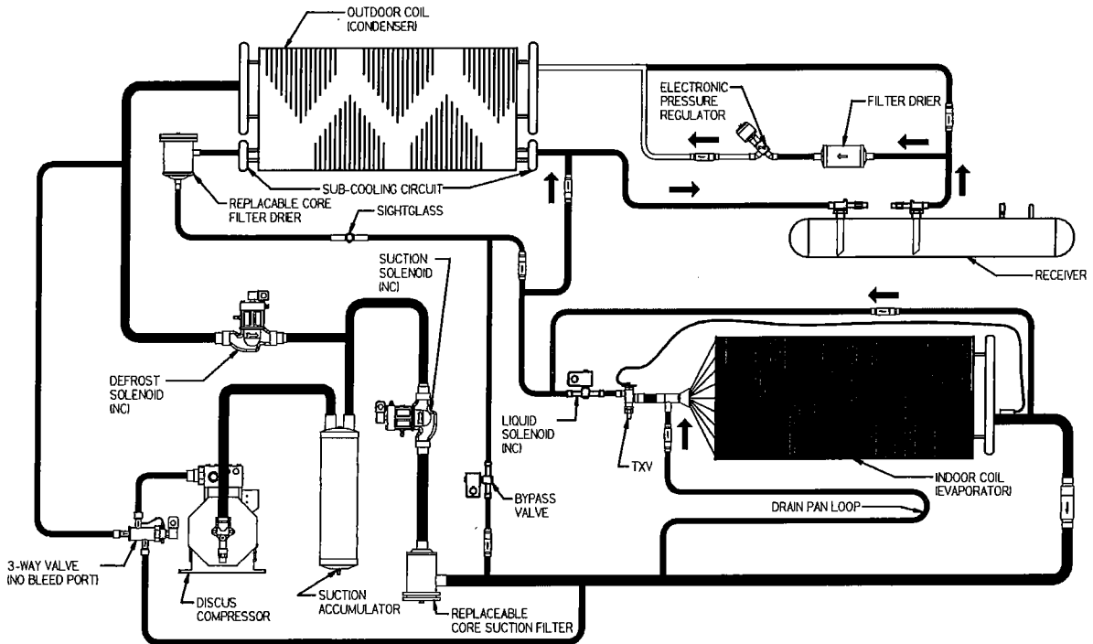
DEFROST-3 MODE
