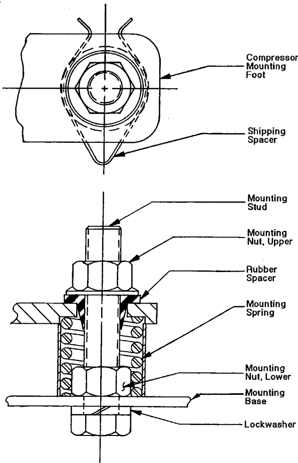
Figure 3. Spring Mount
