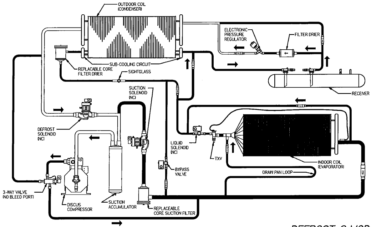
DEFROST-2 MODE
