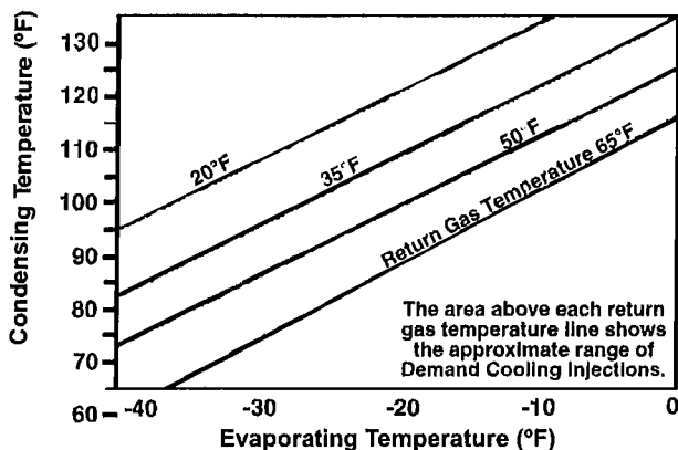
Figure 12. Demand Cooling Injection
