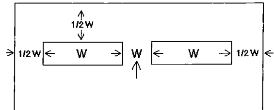
Two evaporators
